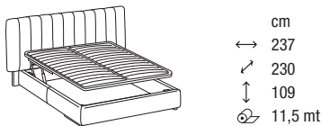
DTMFEX3 DOUBLE BED WITH FLOOR STANDING BED FRAME FOR 180X200 WOODEN SLAT SYSTEM WITH ELEVATED HORIZONTAL MECHANISM
